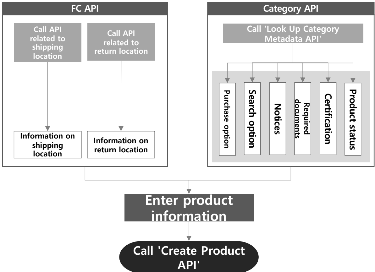
<[Figure] General Flow of the 'Create Product API' Call>
